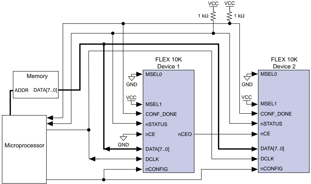
Figure 11. PPS Multi-Device Configuration Circuit
