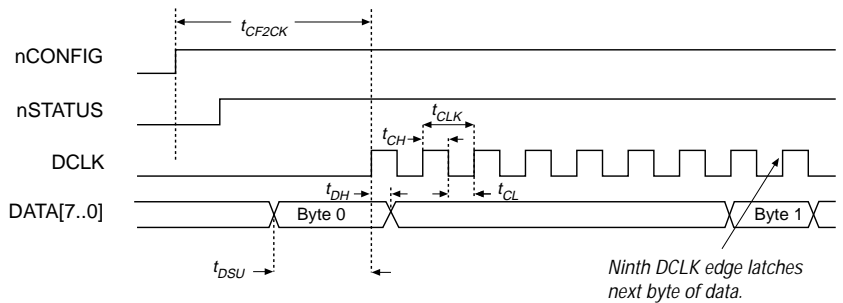
Figure 12. PPS Timing Waveform
