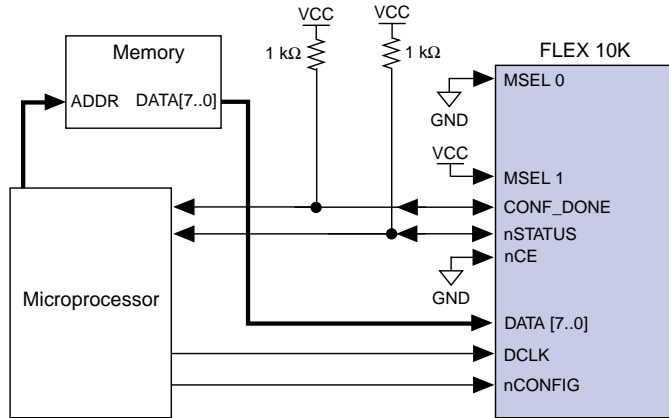
Figure 10. PPS Configuration Circuit
