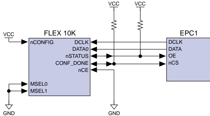
Figure 2. Configuration EPROM Scheme Circuit
