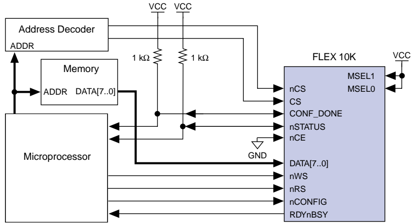
Figure 13. PPA Configuration Circuit
