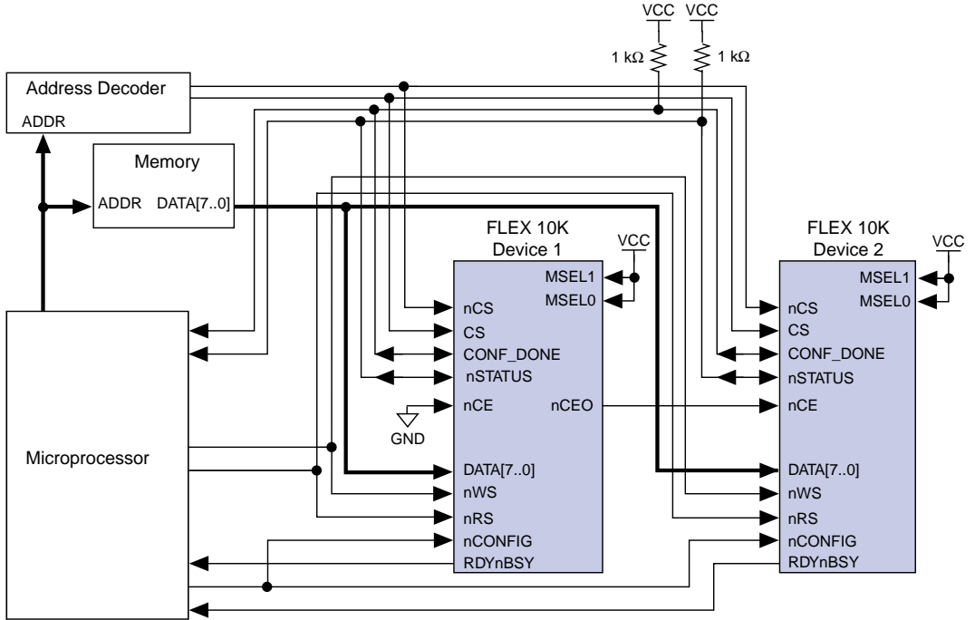
Figure 14. PPA Multi-Device Configuration Circuit
